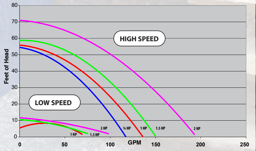
SMF PERFORMANCE CHART
